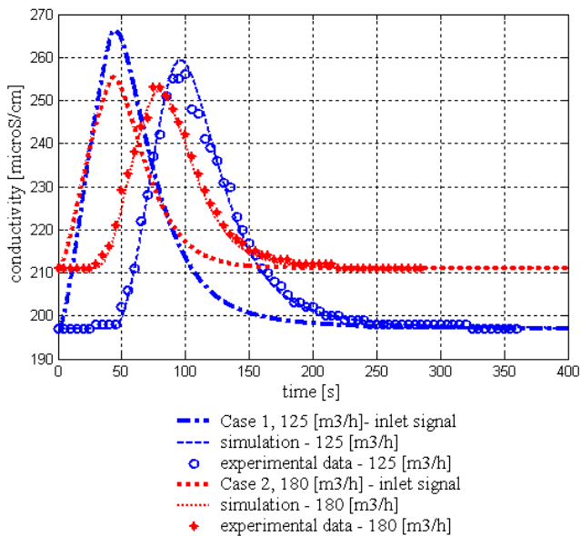
Fig. 4 RTD results for the input to reaction chamber (pipe outlet).
