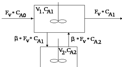
Fig. 2 Chollette-Cloutier model: real mixing model containing steady areas
