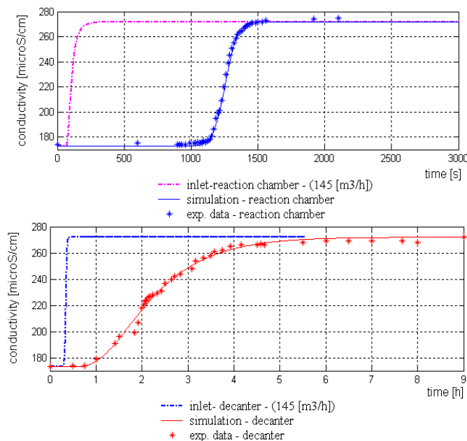
Fig. 7 Reaction chamber and settling tank: experimental results versus validated models predictions at 145 (m 3 /h)
