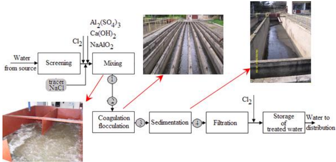
Fig. 1 Process flow diagram of water treatment pilot plant
