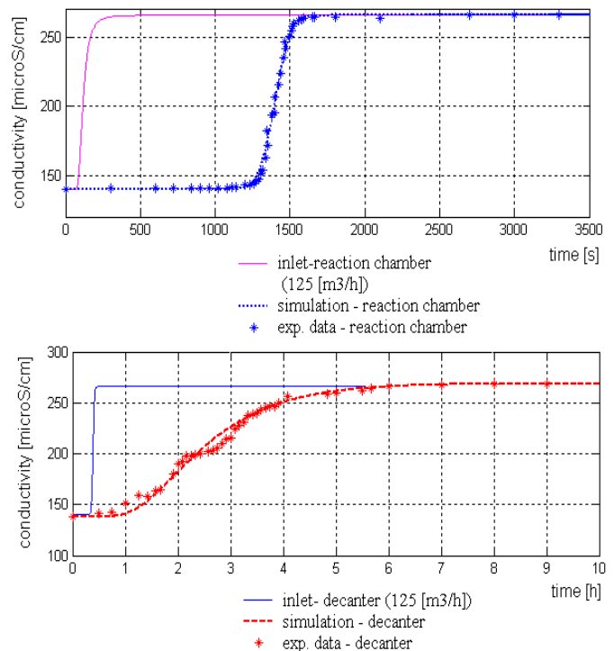
Fig. 5 RTD results for the reaction chamber and settling tank at 125 (m 3 /h). Optimal values of models parameters:
