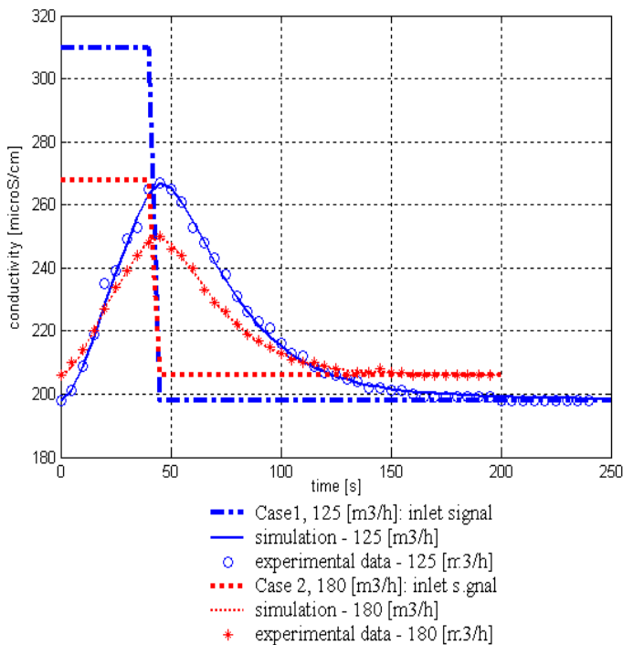
Fig. 3 Typical experimental results for the mixing chamber.
