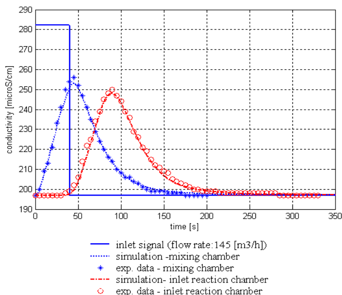
Fig. 6 Mixing chamber and pipe to reaction chamber: experimental results versus models predictions at 145 (m 3 /h)
